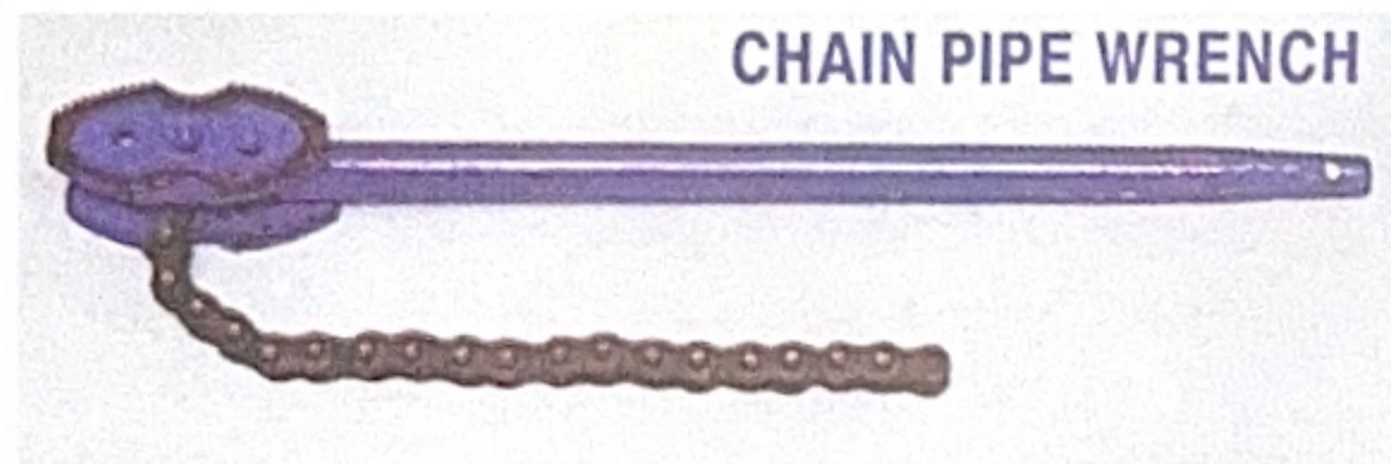
UT-160 : CHAIN PIPE WRENCH SIZE IN INCH. 2, 3, 4, 6, 8, 10, 12
